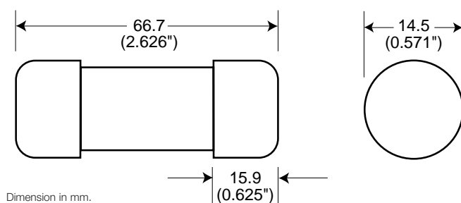
Fig. 1: 20-30 Amp Range
