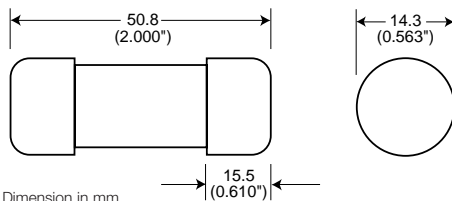
Fig. 1: 1-50 Amp Range
