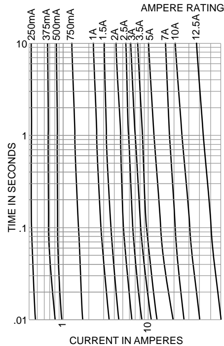
Time-Current Characteristics:
